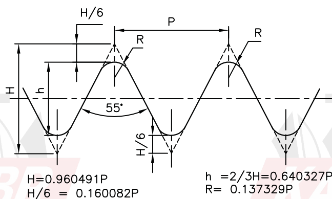
PIPE / G THREAD PROFILE
